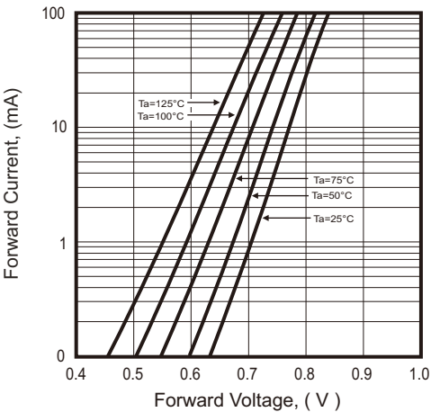
Fig.4 - Forward Characteristic
